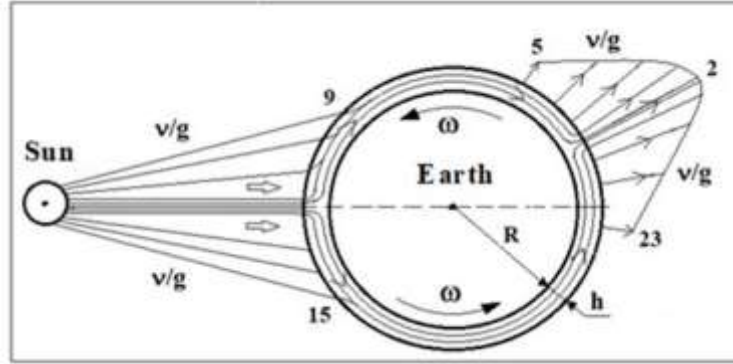
Fig. 3. Diagram of the flow of solar neutrino energy forms ( \nu/g ) over the lithospheric layer h \sim 10 - 50 km thick; number - time of day in hours.
